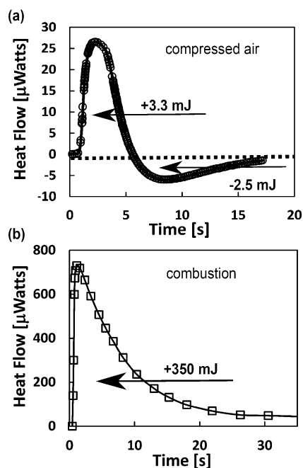
Figure 3. Calorimetric data for a) pneumatic actuation of a pneu-net with a 175 µL chamber volume. The heat produced (exothermic) while pressurizing the chamber by pumping air into the pneu-net (the area under the first curve) is 3.3 mJ; deactuating the pneu-net by sucking air out and depressurizing the chamber is endothermic and absorbs 2.5 mJ of heat (area above the second curve). b) Combustion in the same pneu-net evolves 350 mJ of heat (area under the heat flow versus time curve).
