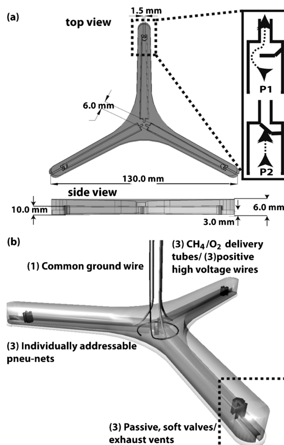
Figure 1. a) Scheme, including dimensions, of a tripod soft robot. Inset: Soft valves allow low pressure (P1) gas to flow out of the exhaust vents in the pneu-net. High pressure (P2) closes the soft valve. b) Rendering of the robot with electrical inputs for spark ignition to actuate the pneu-nets explosively. We fed one wire (a common ground) through each of the pneu-nets, and a separate wire into each channel (a positive terminal for high voltage, three total) to allow independent, timed actuation of each leg. Each of the three high-voltage wires was sheathed in tubing that fed premixed methane and oxygen gas into the pneu-nets.
