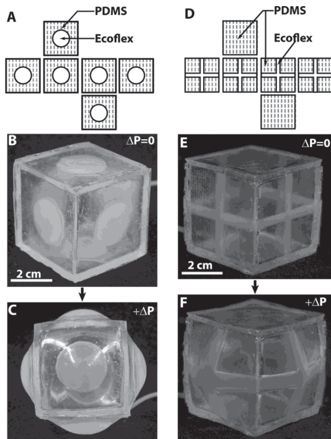
Figure 3. Inflatible cubes fabricated with tiles comprising more than one material. (A, D) Schematic showing the tiles used to fabricate the cube. The PDMS regions of the tile are marked with hatch marks and the Ecoflex regions are solid white. (B, E) Photographs of the actuator with no pressure applied. (C, F) Shape change achieved using positive pressure ( +\Delta P \sim 10 kPa).
